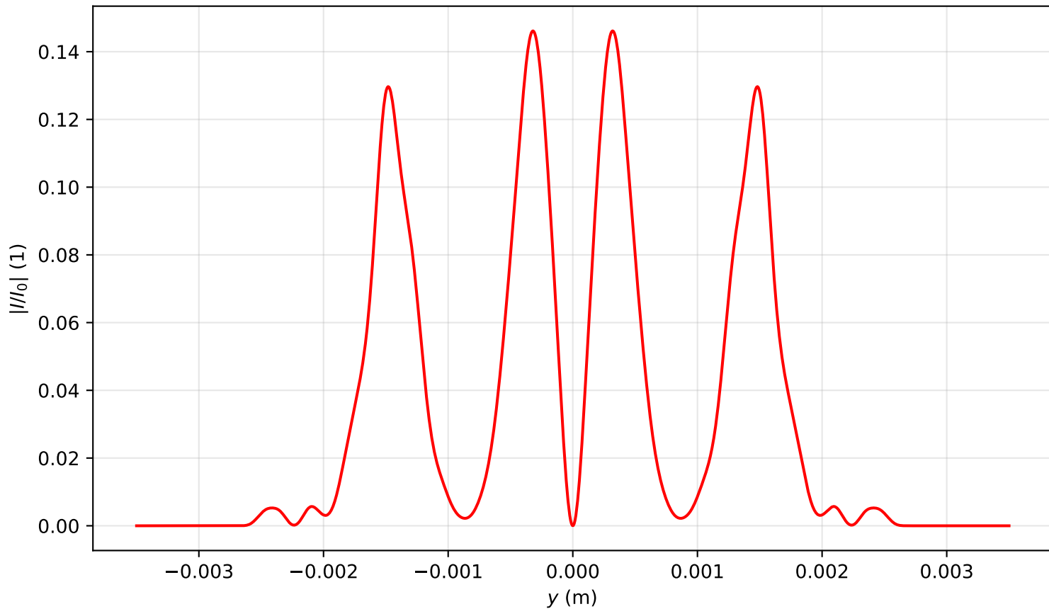
Intensity profile I(x=0, y, z=2.229)/I_0 , P_{in}=9.0P_{cr} , artificial time
